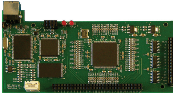
MultiWriter Control Module (-074) Made in U.S.A.
